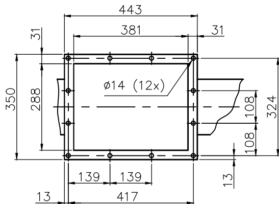
DETAIL "X" SUCTION FLANGE
